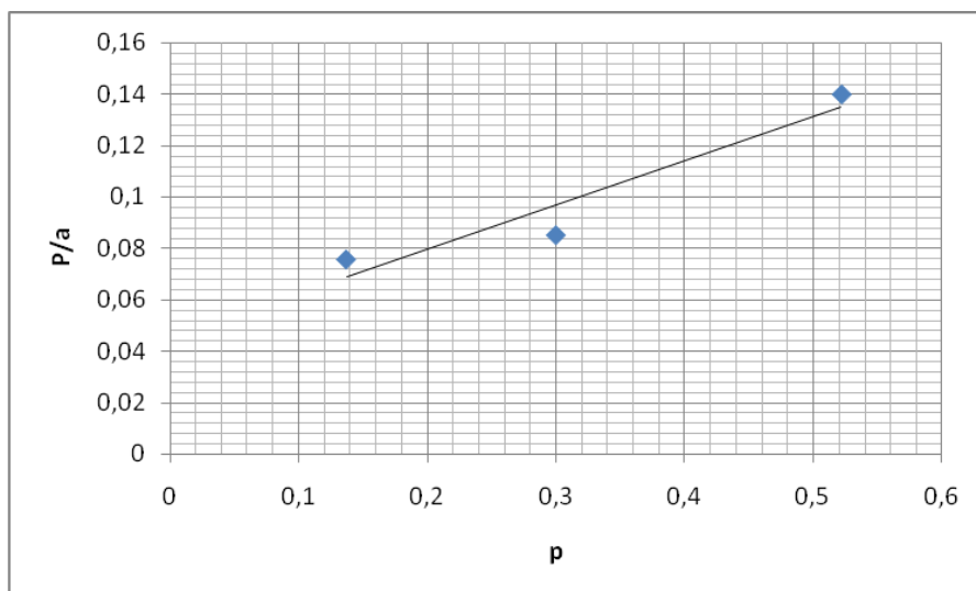
Figure 6. Linear forms of adsorption isotherm in Langmuir coordinates of NH_4NaY + 0.2 \text{ mol/dm}^3 oxalic acid + 1 M p-p HCl
