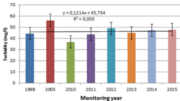
Figure 5b Turbidity
