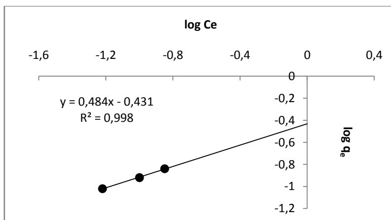
Figure 5. Freundlich adsorption model for Ni(II) on natural bentonite
