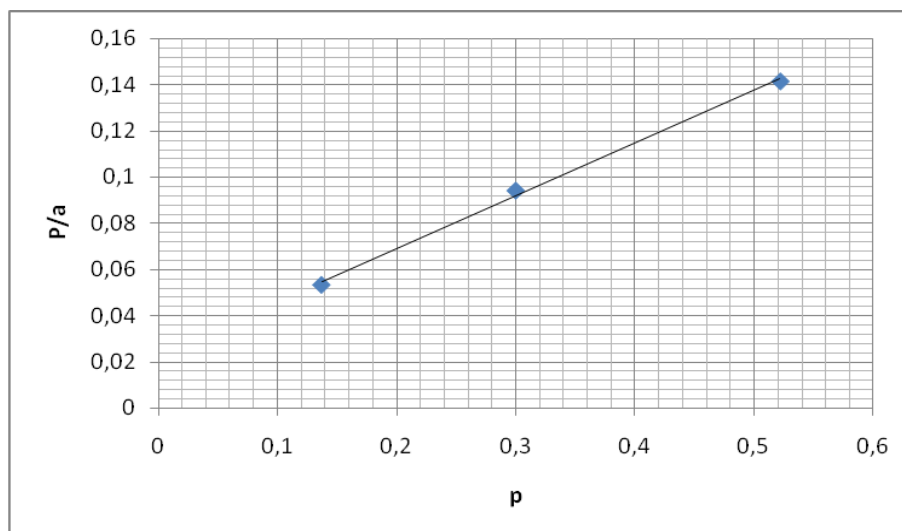
Figure 7. Linear forms of adsorption isotherm in Langmuir coordinates of commercial NH_4NaY zeolite
